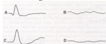
Fig. 4 Primary cortical responses in the cat to acoustic clicks and microwave pulses: A and C are response signals before bilateral destruction of the cochlea. Disablement of both cochlea in the animal resulted in total loss of the responses in the cat to acoustic click (B) and pulsed microwave (D) stimulation. From [48]
