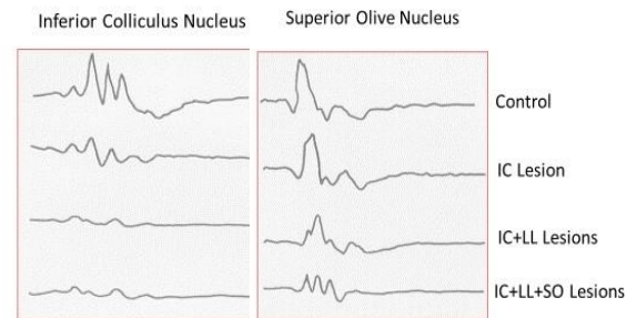
Fig. 8 Effect of successive brainstem ablative lesions on electrical potentials from the inferior colliculus (control) and superior olive nuclei (control) evoked by 25- \mu s wide, 2450 MHz microwave pulses in the cat: Inferior colliculus (IC), lateral lemniscus (LL), superior olive (SO) nuclei. From [45]
