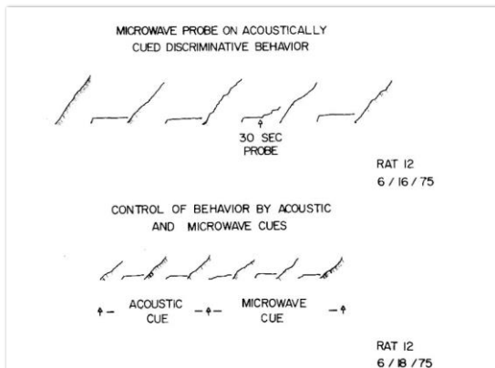
Fig. 2 Cumulative record showing an animal's performance. Top: In response to 30-s microwave probe, rat begins to respond as if acoustic cue had been presented. Bottom: Rat responds equally well during presentation of acoustic and microwave stimulation. From [28]
