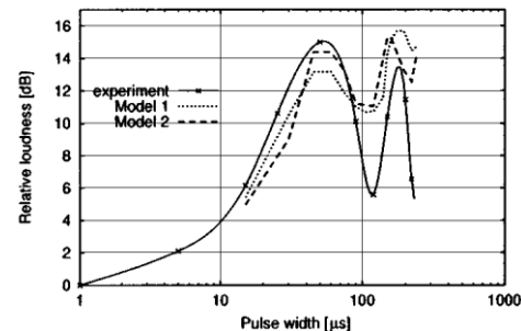
Fig. 1 Loudness of pulse induced sound level as a function of microwave pulse width in human subjects. From [60]
