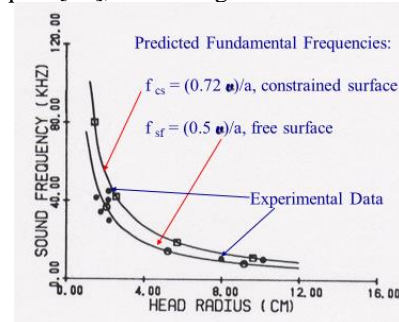
Fig. 9 Theory predicted and experimental measured audible range of frequencies as functions of the subject's head size. From [4]
