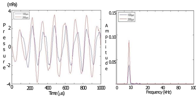
Fig. 10 Computed pressure waves (Left) and amplitude spectra (Right) for an anatomic head model of adult human exposed to 400 MHz microwave pulses of 200- \mu s (Red) and 100- \mu s (Blue) width. From [61]
