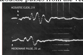
Fig. 3 Brainstem electrical potential responses (BER) from the vertex of a cat's head evoked by acoustic clicks and microwave pulses. From [45]
