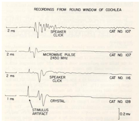
Fig. 6 Carbon electrode recordings from the round window of the cat cochlea elicited by acoustic click and microwave pulse stimuli. From [2]
