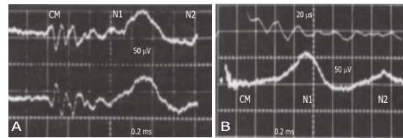
Fig. 7 Cochlear microphonics recorded from round window of the guinea pig. (A upper) Acoustic click stimulus; (A lower) Single 10- \mu s wide, 918 MHz microwave pulse; (B) time expansion of initial 200 \mu s microwave. From [54]
