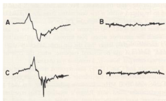
Fig. 5 Acoustic and microwave pulse-evoked responses recorded from the medial geniculate body of a cat. A and C are the corresponding response signals before bilateral destruction of the cochlea. Total loss of the medial geniculate responses in the cat to acoustic click (B) and pulsed microwave (D) stimulation following perforation of both cochlea in the animal. From [48]
